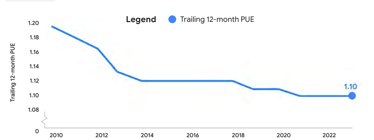
FIGURE 3 Energy efficiency at Google data centers
